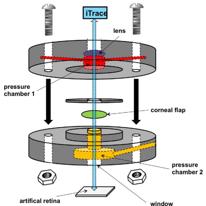
FIGURE 2. Measurement set up.
