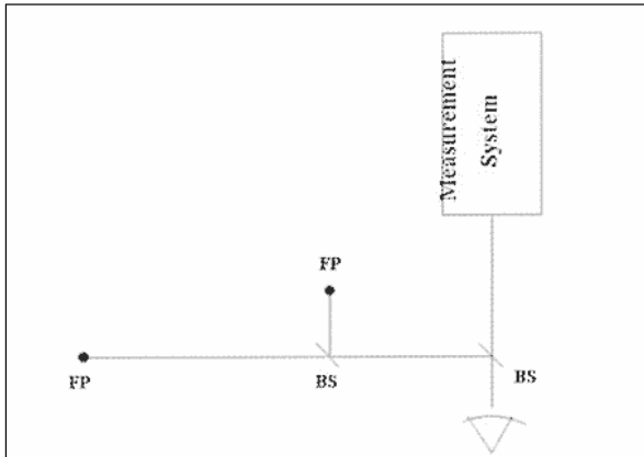
Figure 5. Schematic of a generic subjective alignment system designed to place the line of sight on the optical axis of the measurement system. BS: beam splitter, FP fixation point source.
