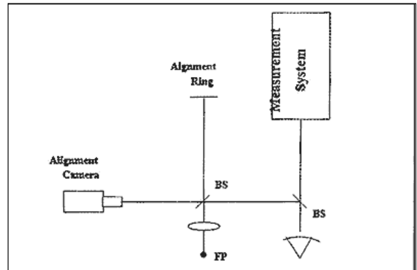
Figure 4. Schematic of a generic objective alignment system designed to place the line of sight on the optical axis of the measurement system. BS: beam splitter, FP: on axis fixation point.
